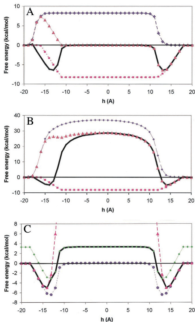
FIGURE 3 (A and B) The translocation of valproic acid (A) and valproate (B) across the lipid bilayer, in the orientation of Fig. 1. The electrostatic (◆), nonpolar (■), and solvation (▲) free energies of the VPA-membrane system are presented as a function of the distance h between the geometrical center of the molecule and the membrane mid-plane. The solid line in A and B presents an alternative flip-flop path, in which VPA reverses its orientation in the membrane by a 180° rotation after the complete insertion of the carboxyl group inside the bilayer. (C) The minimal free energy path for the flip-flop of valproate across the membrane. ▲, \Delta G_{\text{sol}} for the flip-flop of valproate in its charged form, taken from B; ●, \Delta G_{\text{sol}} for the flip-flop of valproic acid (neutral form), taken from A; ◆, sum of \Delta G_{\text{pKa}} (the free energy of discharging valproate in the aqueous phase) and \Delta G_{\text{sol}} for its flip-flop in the neutral form. The solid line denotes the minimal free energy path for the flip-flop of (negatively charged) valproate across the membrane. Note the curve crossing at h = -13.5 Å and h = 13.5 Å, where the valproate becomes protonated to reduce the free energy of translocation across the membrane. The zero of the free energy was chosen at h = \infty . The membrane width was 30 Å. The calculations were carried out on a lattice of 65^3 points with a resolution of 3 grid points per Å as described in Materials and Methods.
